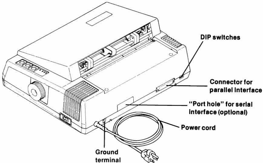
Figure 1-2. The connectors and DIP switches are located on the back of the Gemini printers.
