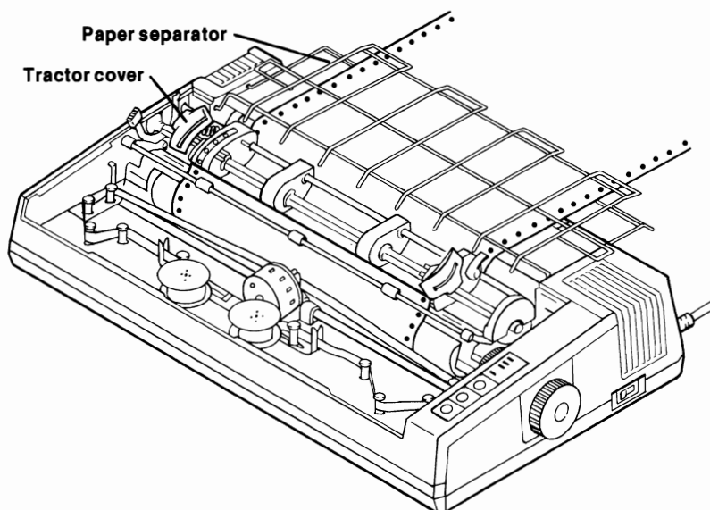
Figure 2-12. The Gemini-15X can be loaded with sprocket paper from the back (as shown here) or from a stack of paper beneath the printer (depicted in Figure 2-13).
